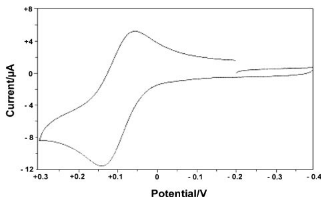
Figure 3. Cyclic voltammogram for the [\text{NEt}_4][\{\text{Mo}(\text{CO})_2(\eta^3\text{-C}_3\text{H}_5)_2(\mu\text{-OC}_6\text{H}_4\text{CH}_3)_3\}] ( 4a ) complex.
