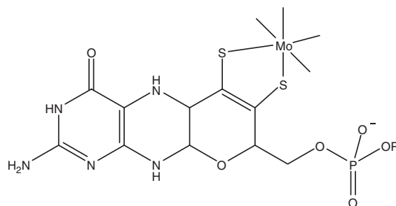
Figure 1. Molybdenum oxotransferase and hydroxylase enzyme cofactor.
