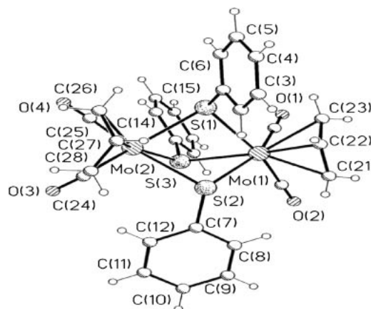
Figure 2. X-ray structure of the [\text{NEt}_4][\{\text{Mo}(\text{CO})_2(\eta^3\text{-C}_3\text{H}_5)_2(\mu\text{-SC}_6\text{H}_5)_3\}] ( 3a ) complex.
