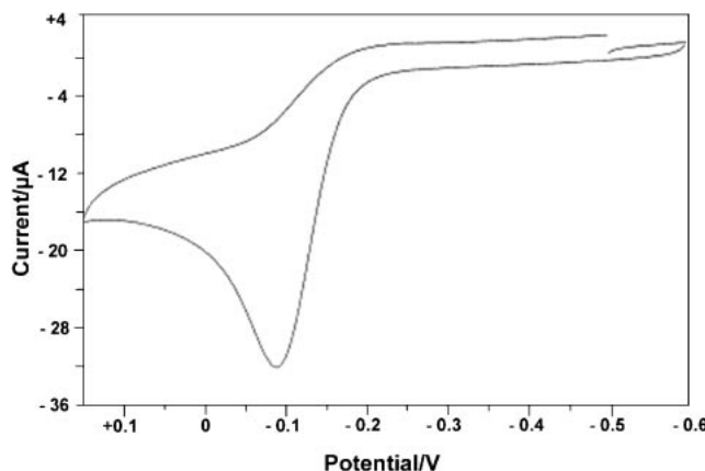
Figure 4. Cyclic voltammogram for the [\text{NEt}_4][\{\text{Mo}(\text{CO})_2(\eta^3\text{-C}_3\text{H}_5)_2(\mu\text{-SC}_6\text{H}_5)_3\}] ( 3a ) complex.
